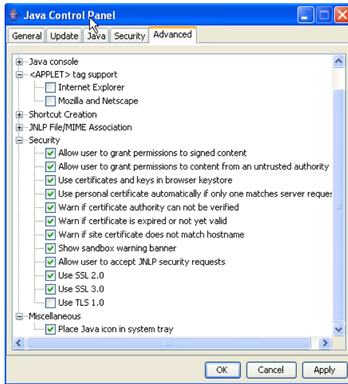
Figure 2-13: Java Control Panel Settings
