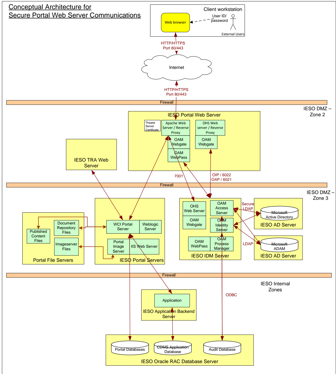
Figure 2-20: IESO Portal Conceptual Architecture
