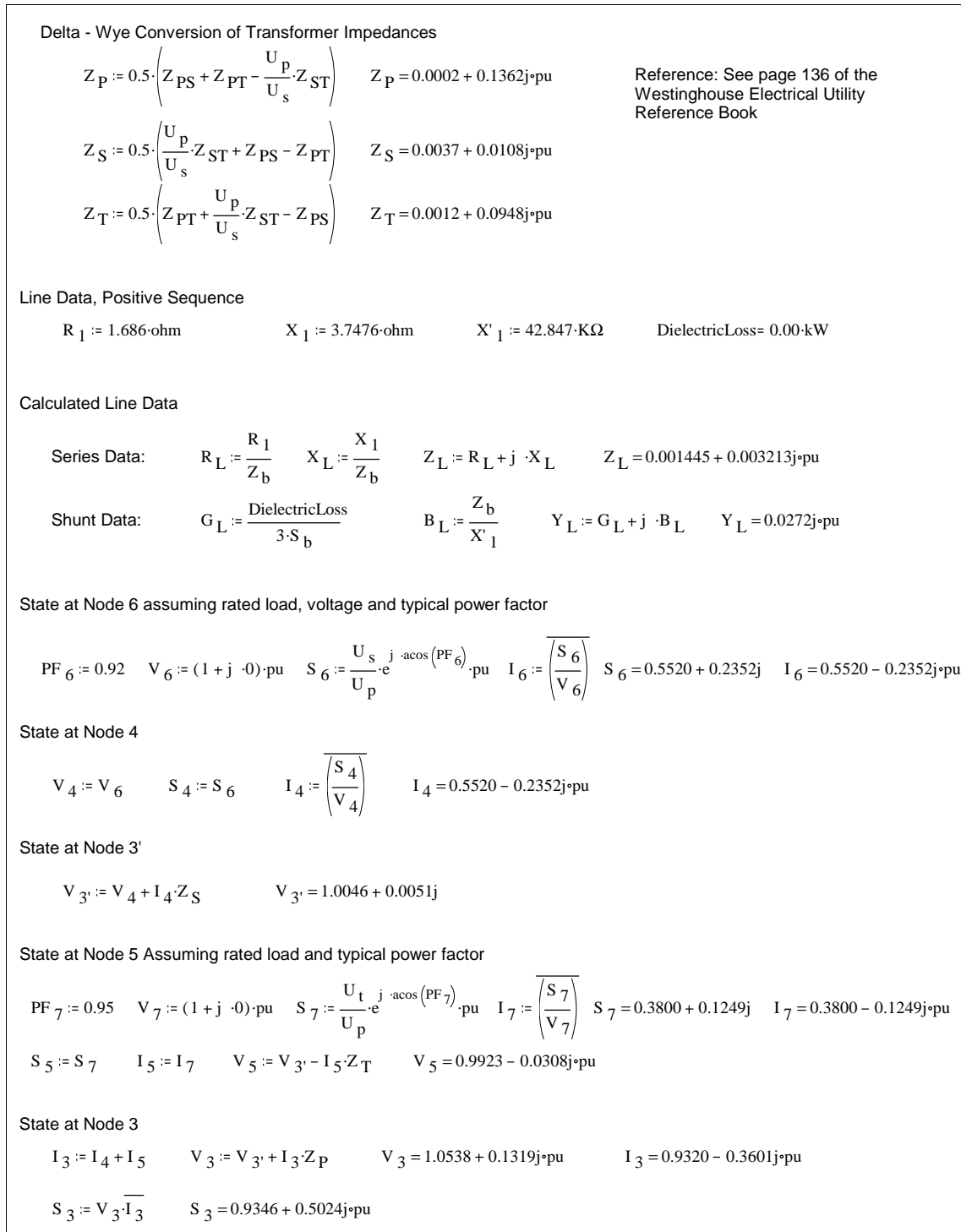
Figure B.2: Application of Method 2 to a three-winding power transformer (continued)
