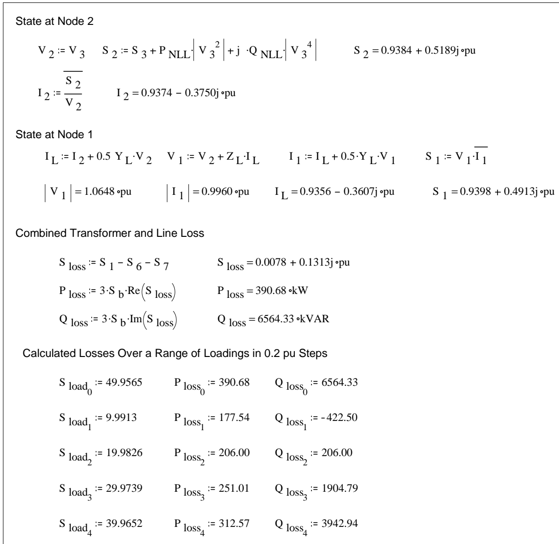
Figure B.3: Application of Method 2 to a three-winding power transformer (continued)
