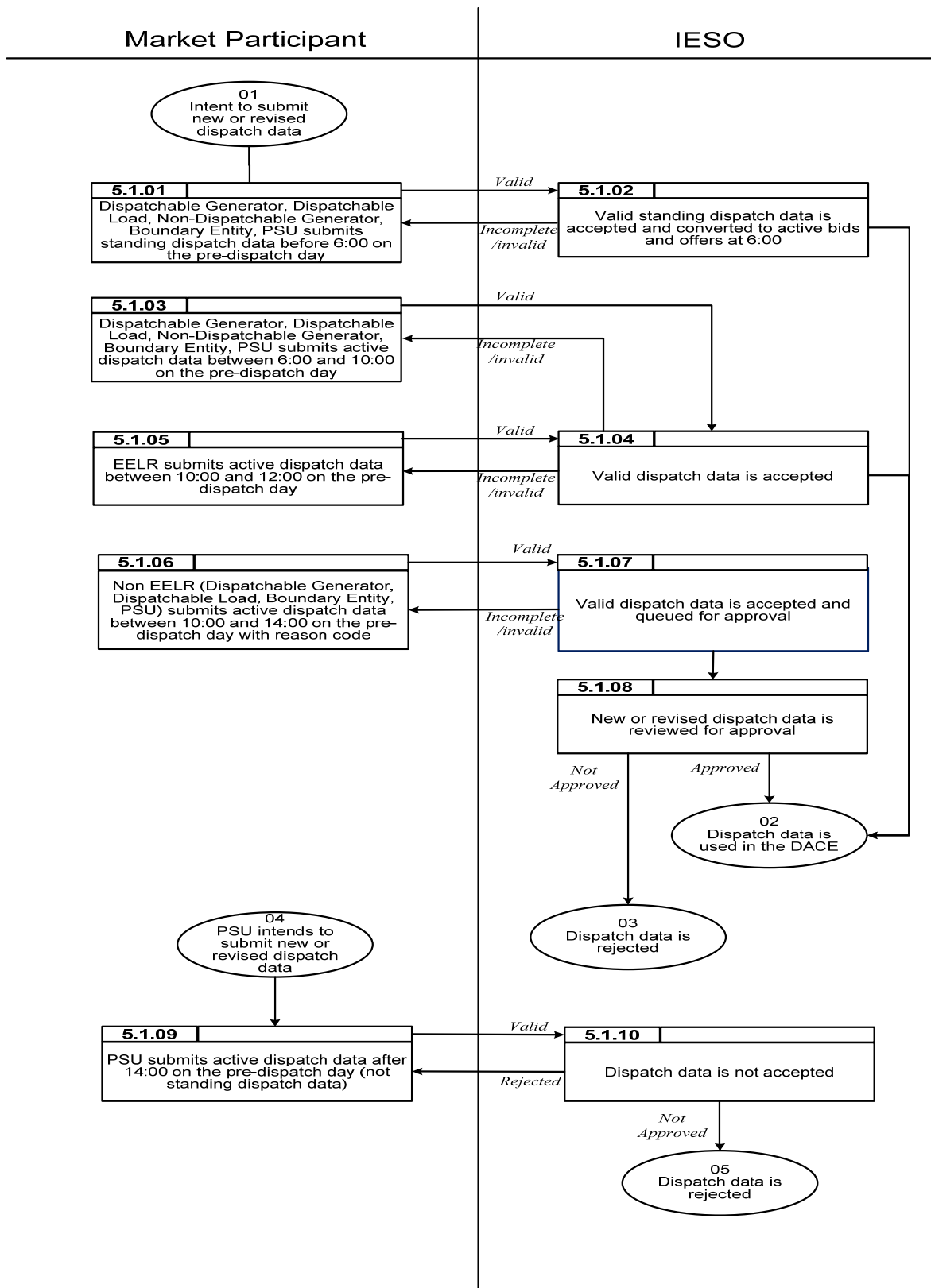
Figure 5-2: Workflow for Submit New or Revised Dispatch Data
