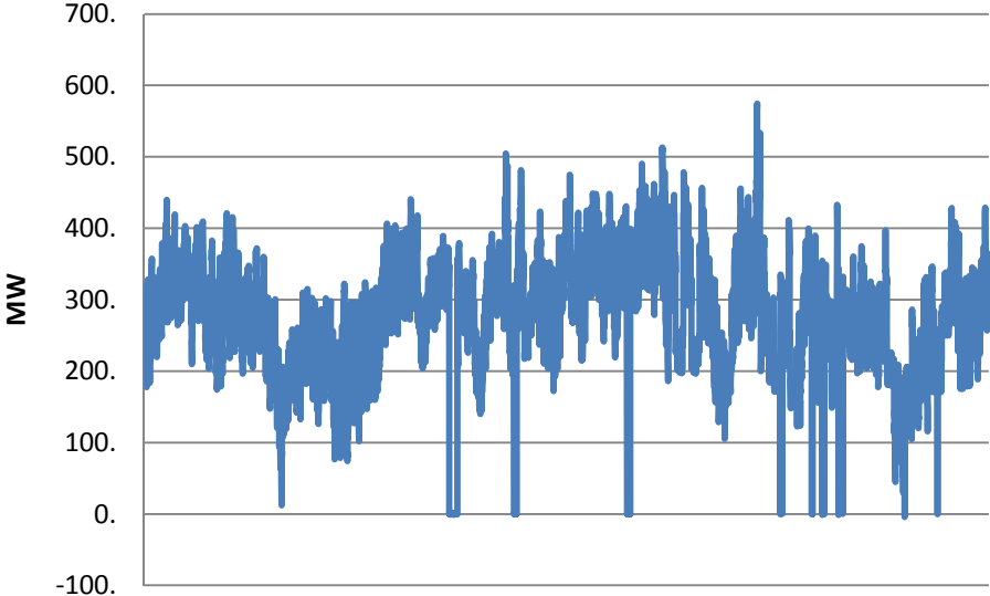
Figure 4: MW flow on W45LC at Longwood TS
