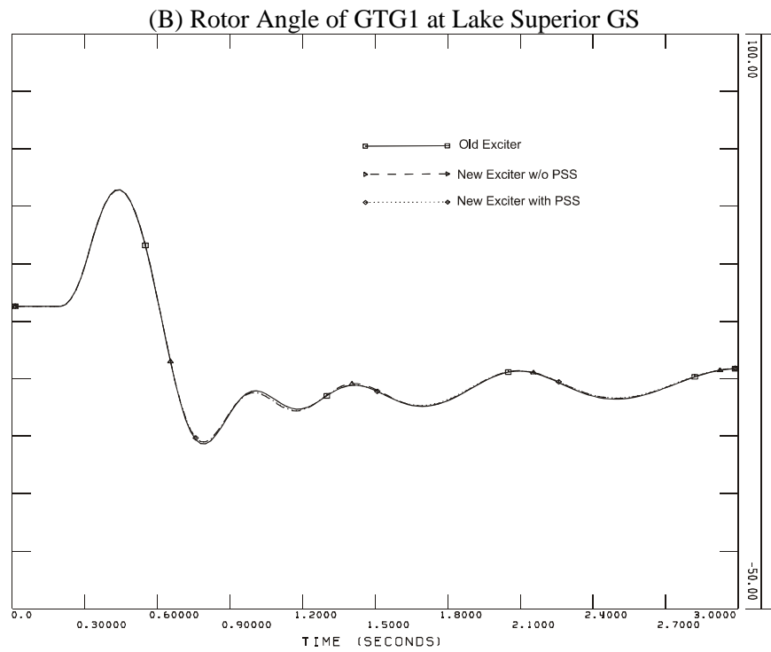
Figure 5 Simulation Results for a LLG Fault
